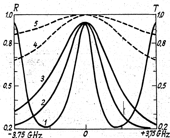
FIG. 2. Frequency-selective loss functions: T(\nu) for Fabry-Perot etalons with a base line of 10 mm, R_{1,2} = 0.04 , (curve 5) and R_{1,2} = 0.1 (4); R(\nu) for a selective reflector with an absorbing film with a film-mirror distance of 4 (1), 2 (2), and 4/3 cm (3).
