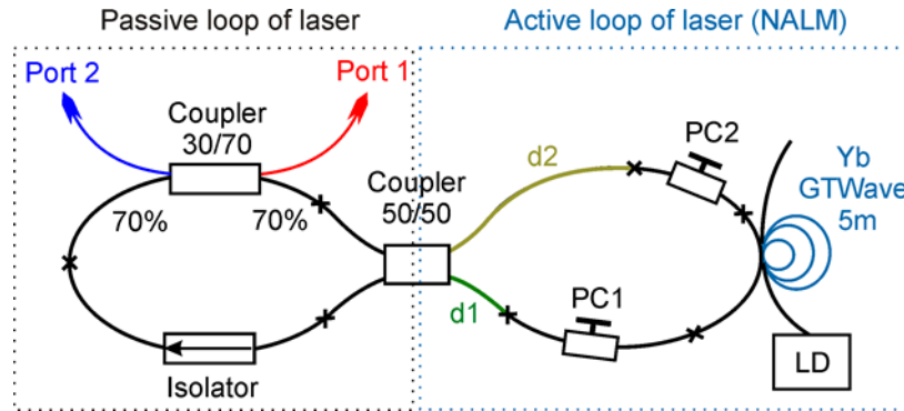
Fig. 1. Experimental layout: PC1, PC2 – polarisation controllers; LD – pump laser diode; d1, d2 – stretches of polarisation-maintaining fibre.
